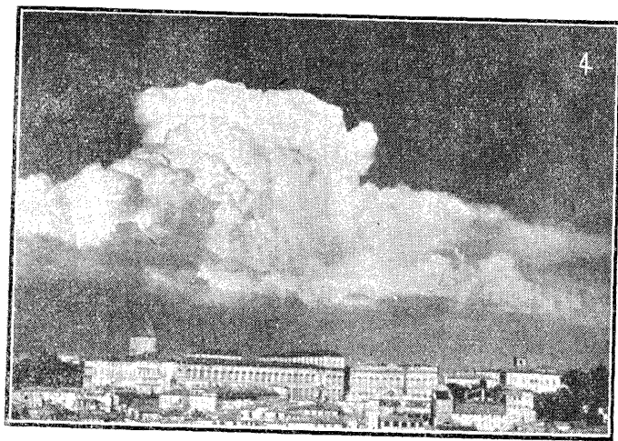
3. Alto-cumulus, — 4. Cumulus (compositus)
